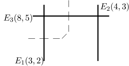
Figure 2: Intersection diagram of the principalization of (x^4, xy^2, y^3) .
