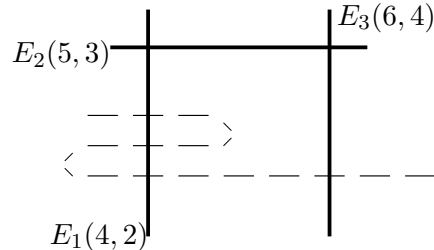
Figure 1: Intersection diagram of the principalization of (x^3y, x^6 + y^4) .
