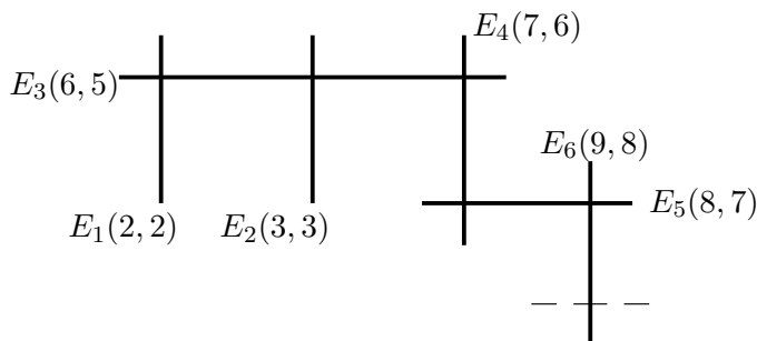
Figure 3: Intersection diagram of the principalization of (x^3y, x^3 - y^2) .
