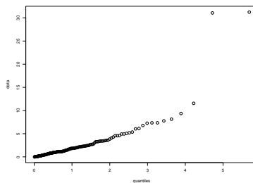
Figure 9: The Baseball data: \chi_2^2 based QQ-plot of the robust distances.
